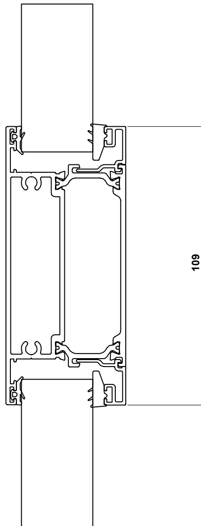
ETD030 - Midrail ETC161 - 28mm Glazing Bead
